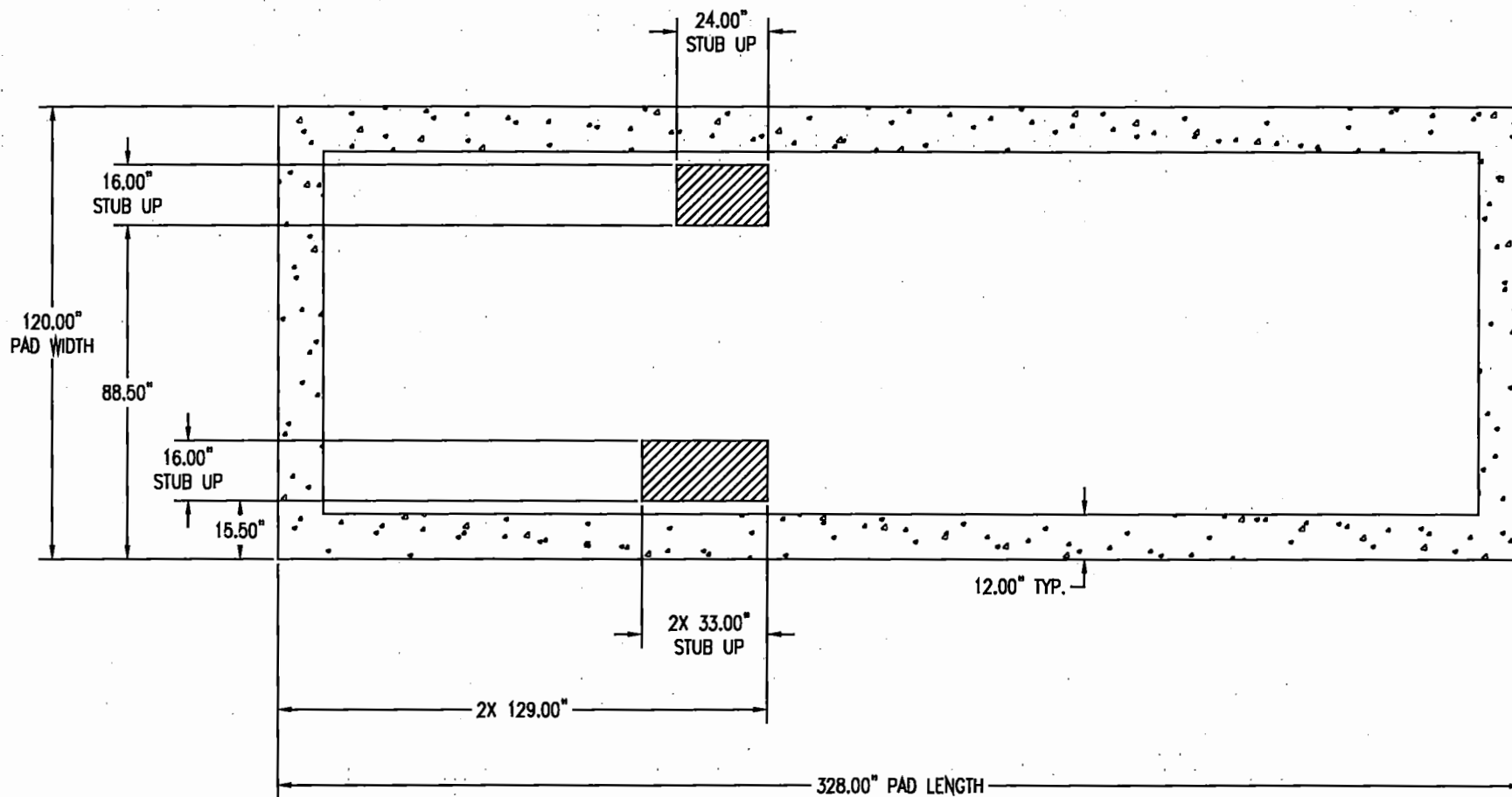
SUGGESTED PAD LAYOUT
